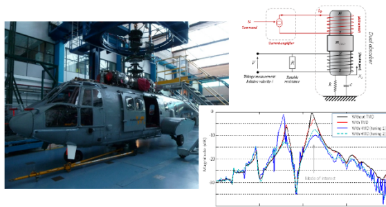
Hybrid Mass Damper: Application to a helicopter
